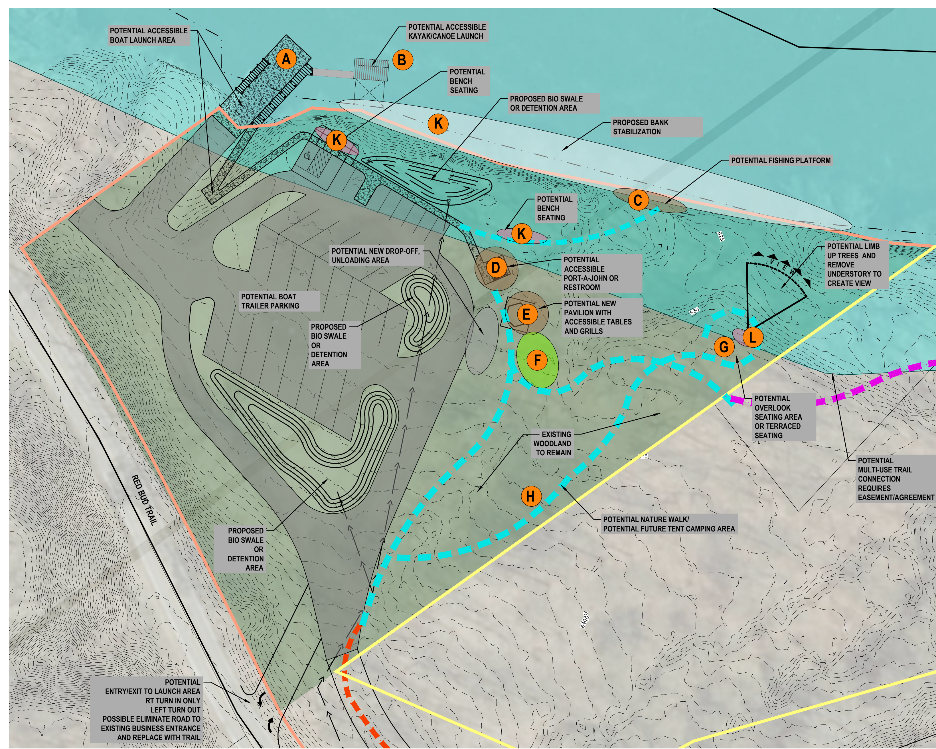
ENLARGED LANDINGS AREA - CITY OWNED SCALE: 1" = 40'
